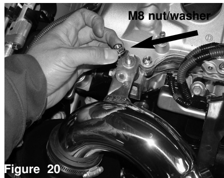
Figure 20 Place a M8 nut and washer onto the vibramount
