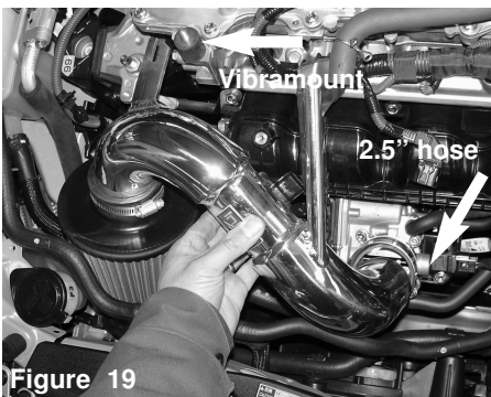
Figure 19 Lower the intake tube into the engine bay and push the non-filter end of the tube into the 2.50" straight hose. Then align the mounting bracket onto the vibramount
