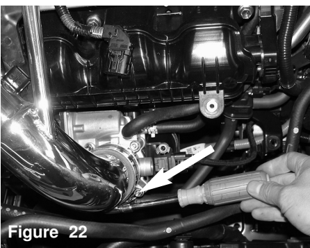
Figure 22 Tighten the second clamp to secure the intake pipe on the 2.5" hose that was already on the throttlebody
