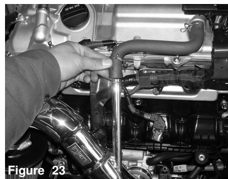
Figure 23 Place the factory breather line to the long 5/8 nipple welded to the pipe.
