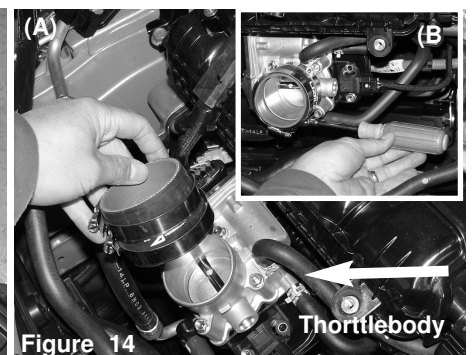
Figure 14 Figure A: Place the 2.5" straight hose and two .040 clamps onto the throttlebody. Figure B: Use a 8mm nut driver to tighten the throttlebody clamp for now.
