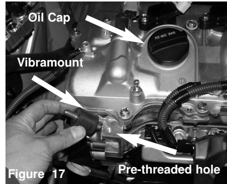
Figure 17 Place the M8 vibramount onto the pre-threaded hole next to the valve cover. Use the oil cap in the photo to reference the location of the pre-threaded hole
